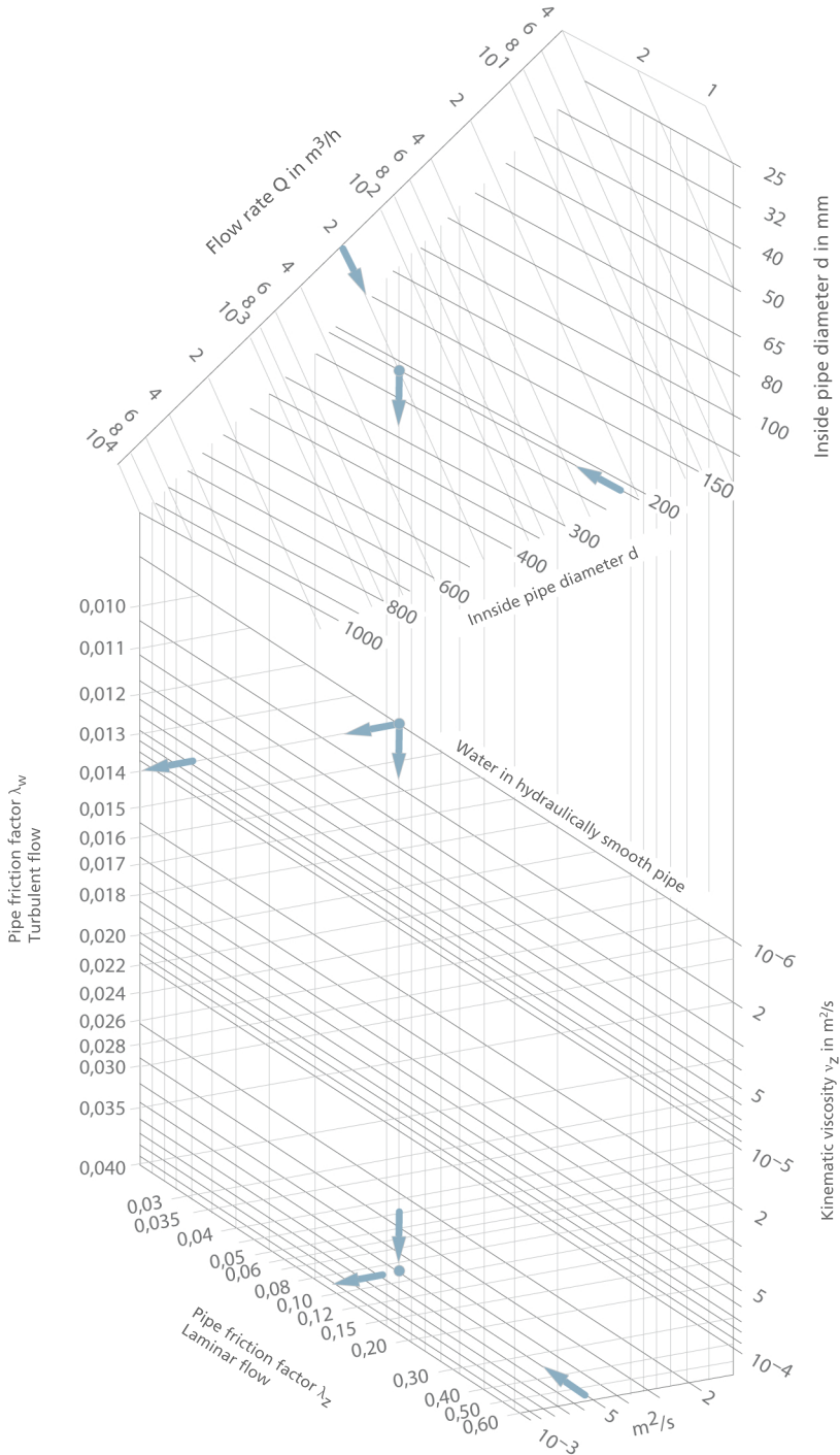
Fig. 13 Head loss: Establishing the pipe friction factor \lambda_z for fluids of higher viscosity. Example: Q=200 m^3/h , d=210 mm , \nu_z=5 \times 10^{-4} m^2/s , \lambda_z=0.09
