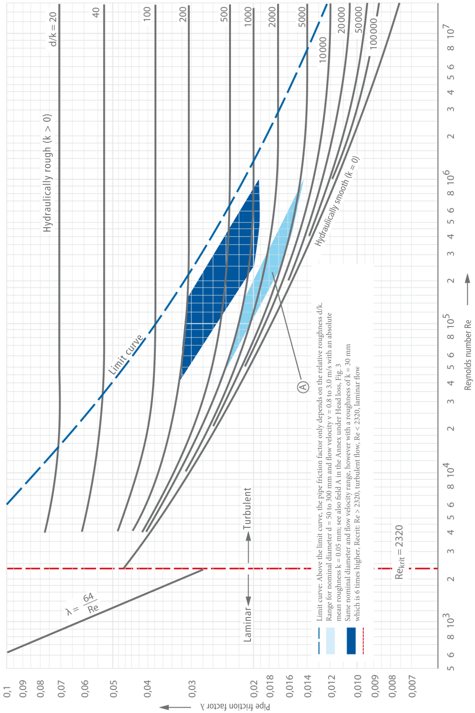
Fig. 1 Head loss: Pipe friction factor as a function of Reynolds number Re and of relative roughness d/k
